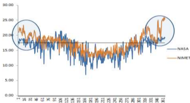
Fig. 5: Comparison of NIMET and GEOS Irradiance Datasets (Annualised)
