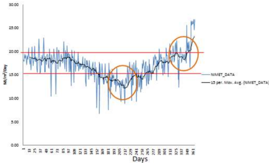
Fig 7: Upper- and Lower-Level Solar Irradiance Benchmarks
